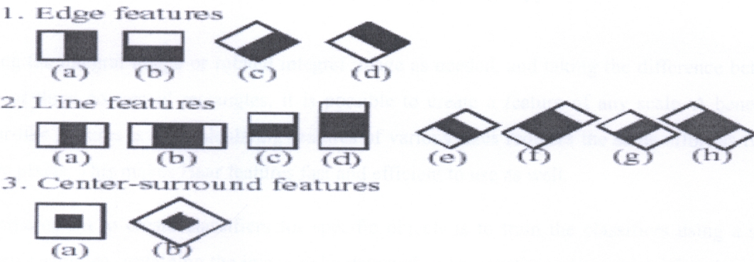
Figure 4.0 Haar-like features
