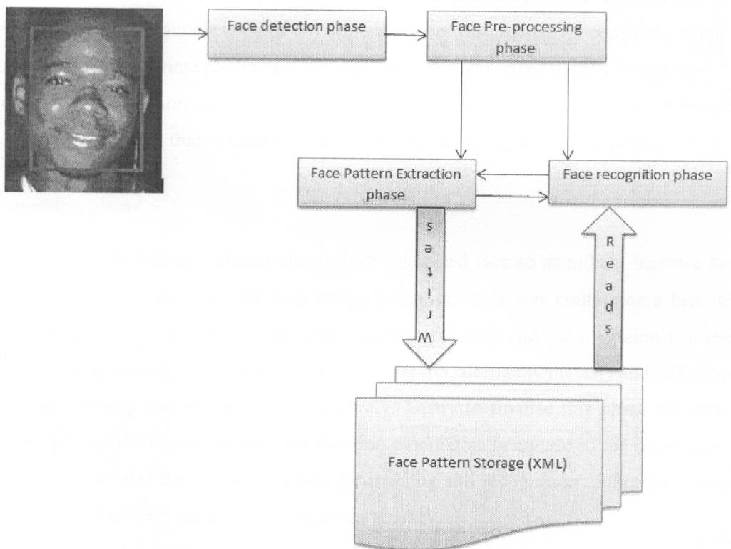
Figure 4.2 face recognition component overview
