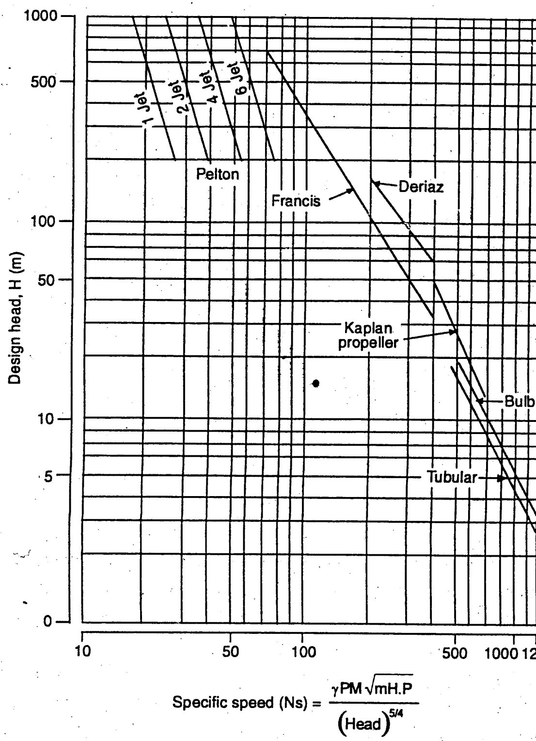
Relation between head and specific speed (IS: 12837-198
