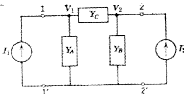
(a) Pi circuit
