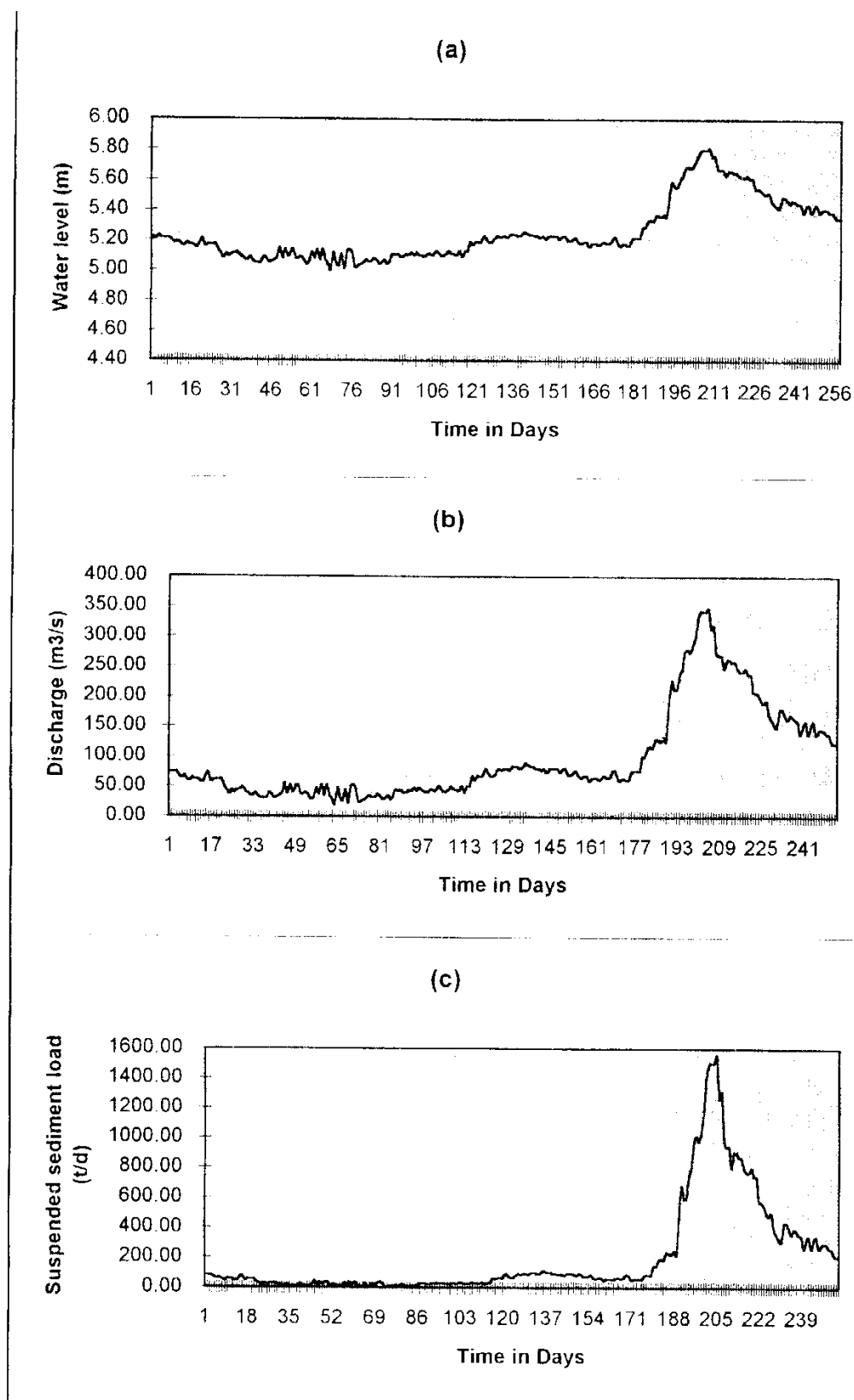
Figure 19. Graphs showing variations in (a) water levels, (b) discharge, and (c) suspended sediment load for Lufubu River at Kabyolwe Village, 16 September 1998 - 31 May, 1999.
