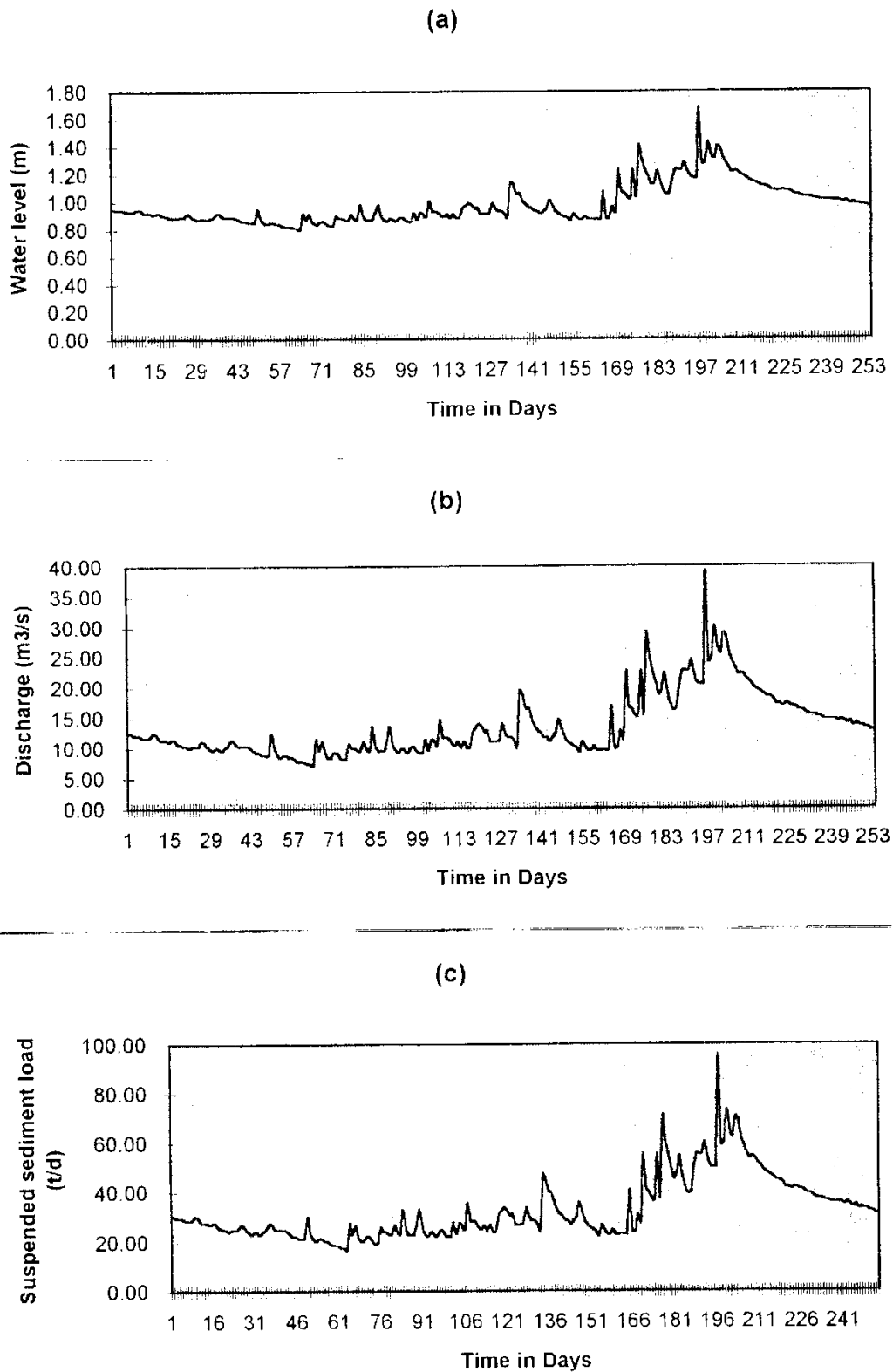
Figure 17. Graphs showing variations in (a) water levels, (b) discharge, and (c) suspended sediment load for Lunzua River at Simumbele Village, 20 September 1998 - 31 May, 1999.
