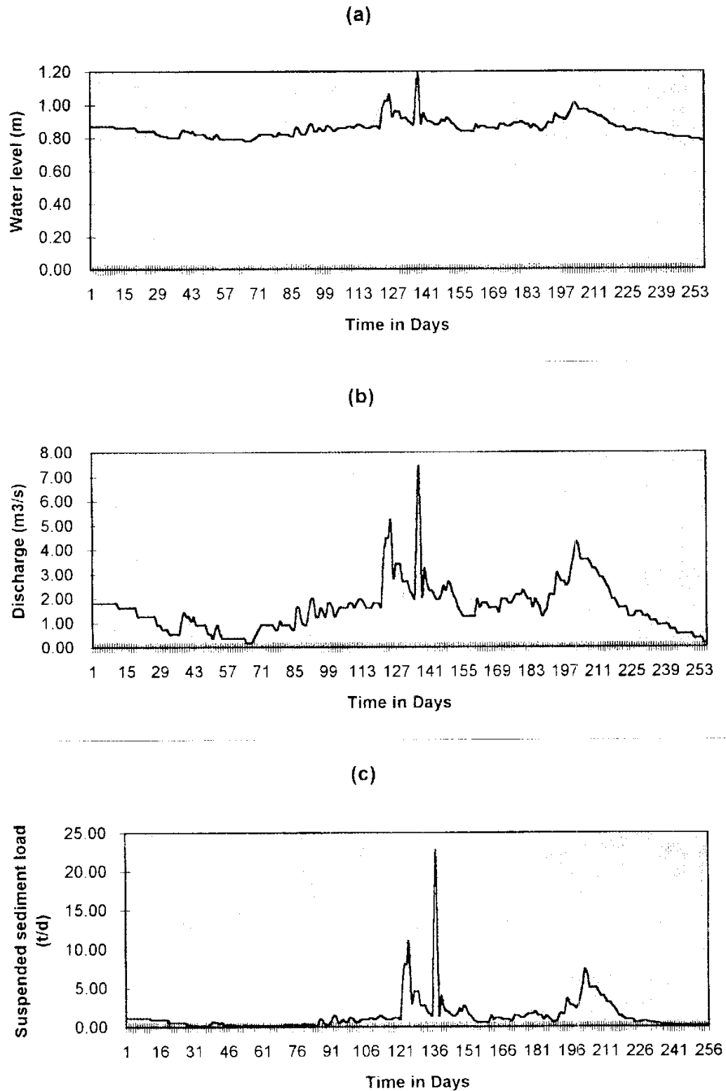
Figure 12. Graphs showing variations in (a) water levels, (b) discharge, and (c) suspended sediment load for Lucheche River at Kawe Village, 17 September 1998 - 31 May, 1999.
