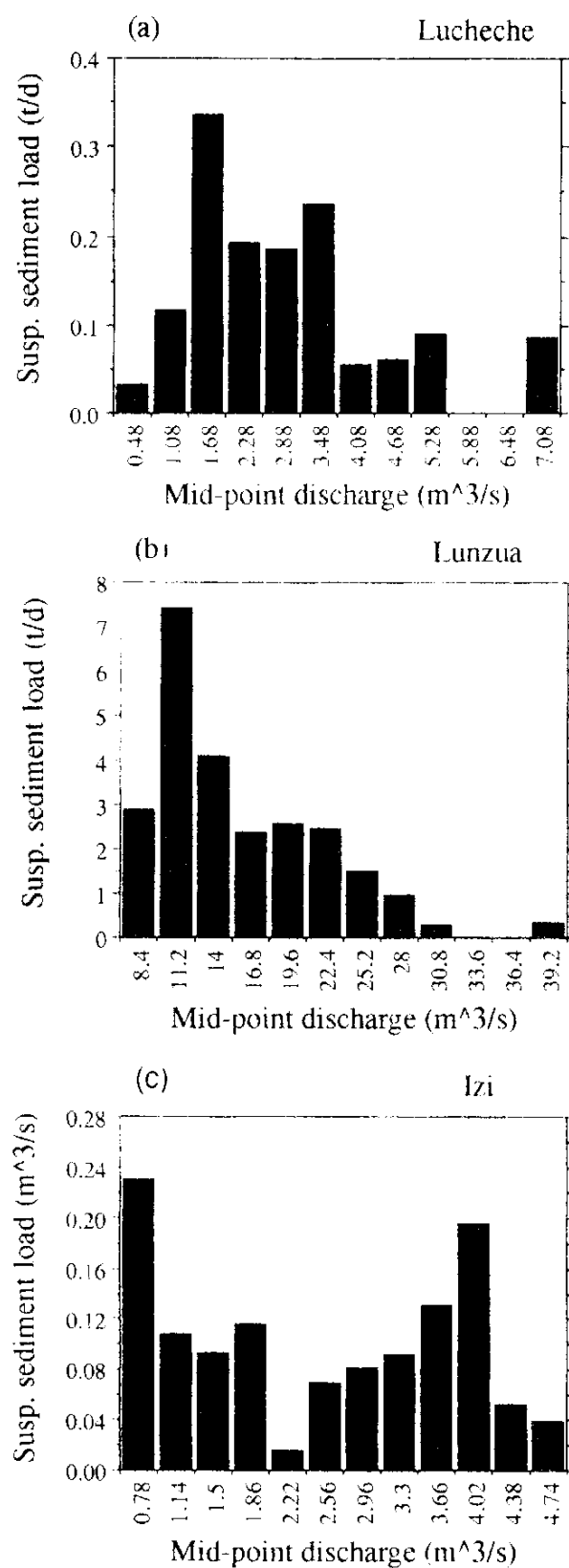
Figure 21. Sediment-discharge regimes for (a) Lucheche River at Kawe Village, (b) Lunzua River at Simumbele Village, and (c) Izi River at Mbete Village, September 1998 - May 1999.
