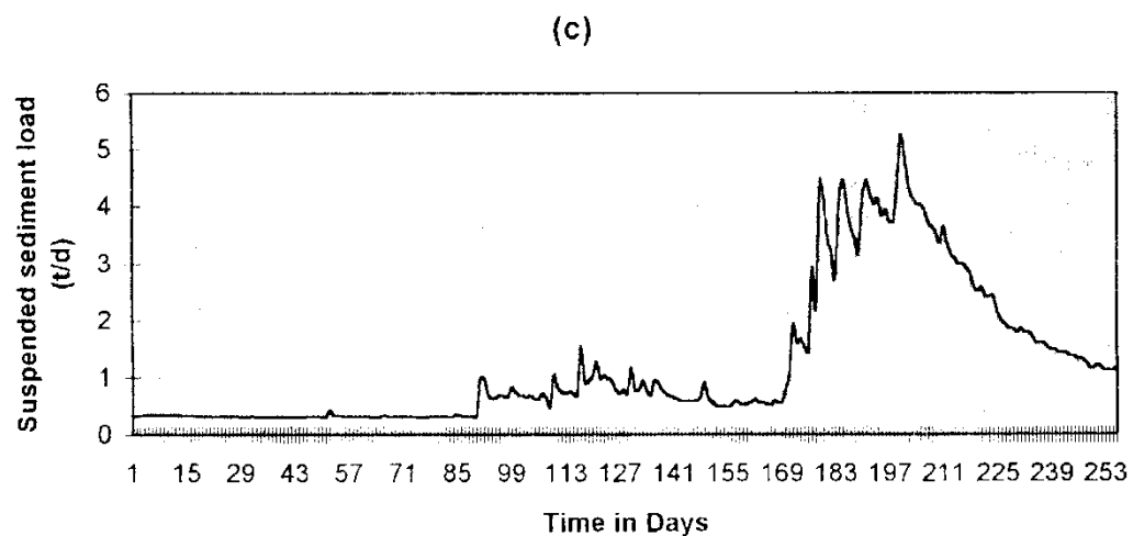
Figure 16. Graphs showing variations in (a) water levels, (b) discharge, and (c) suspended sediment load for Izi River at Mbete Village, 18 September 1998 - 31 May, 1999.
