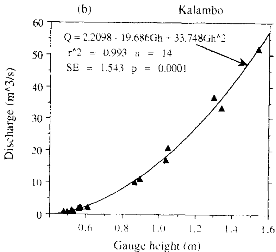
Figure 10 Discharge rating curves for (a) Lucheche River at Kawe Village, and (b) Kalambo River at Kalambo Village, September 1998 - May 1999.
