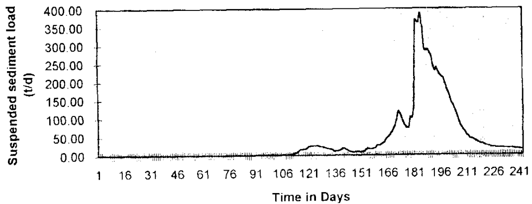
Figure 13. Graphs showing variations in (a) water levels, (b) discharge, and (c) suspended sediment load for Kalambo River at Kalambo Village, 1 October 1998 - 31 May, 1999.
