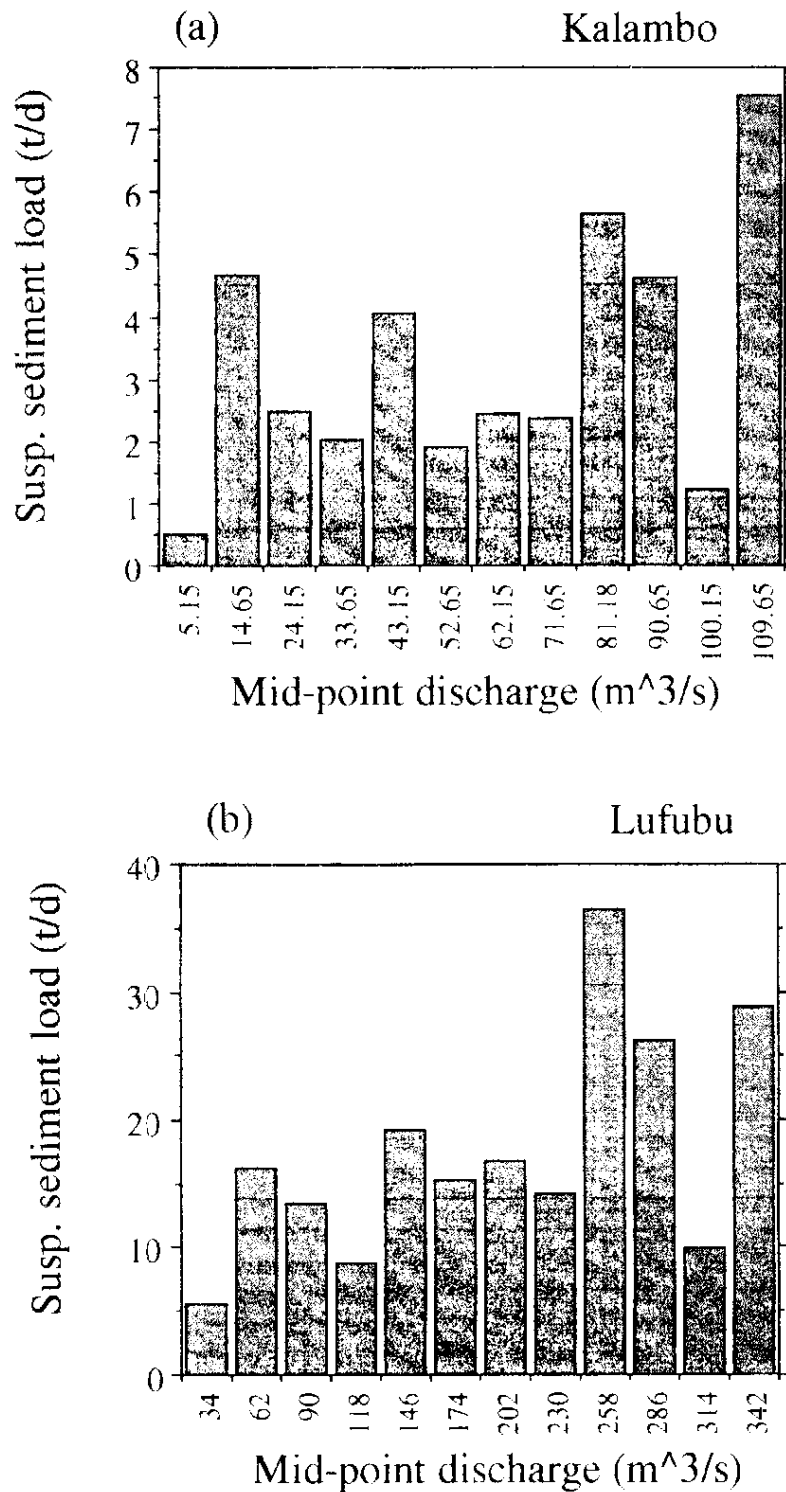
Figure 22. Sediment-discharge regimes for (a) Kalambo River at Kalambo Village, and (b) Lufubu River at Kabyolwe Village, September 1998 - May 1999.
