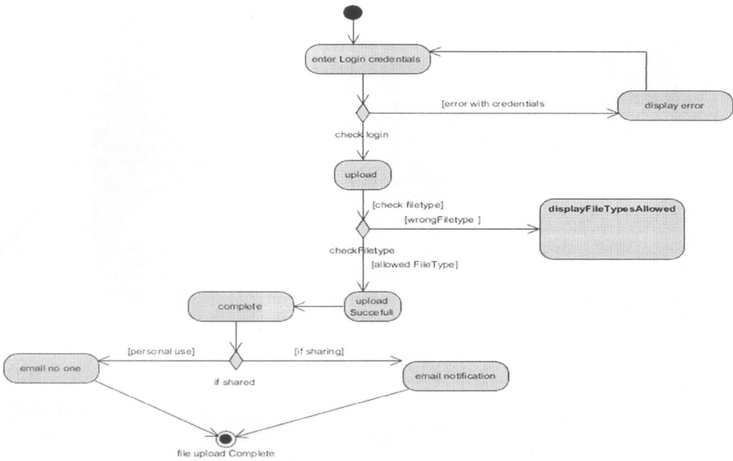
Figure 13 : activity diagram
