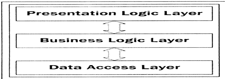
Figure 9 : 3tier architecture
