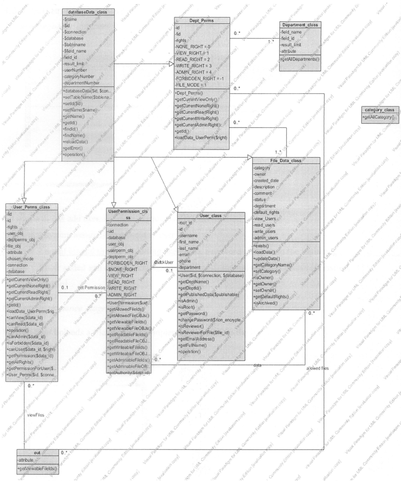
Figure 14 : class diagram
