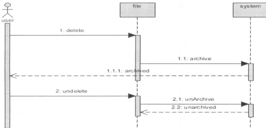
Figure 17 : Delete File Sequence Diagram
